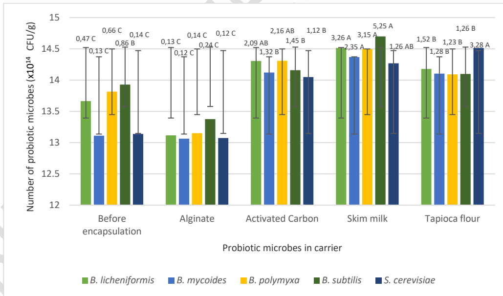
Fig. 3. Number of probiotics (CFU/g) Bacillus licheniformis , B. mycooides , B. polymyxa , B. subtilis , and Saccharomyces cerevisiae before and after encapsulation in alginate, activated carbon, skim milk and tapioca.
