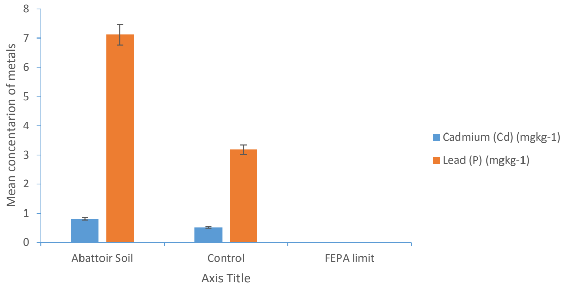
Fig. 3. Concentration of Cadmium and Lead in the soil samples
