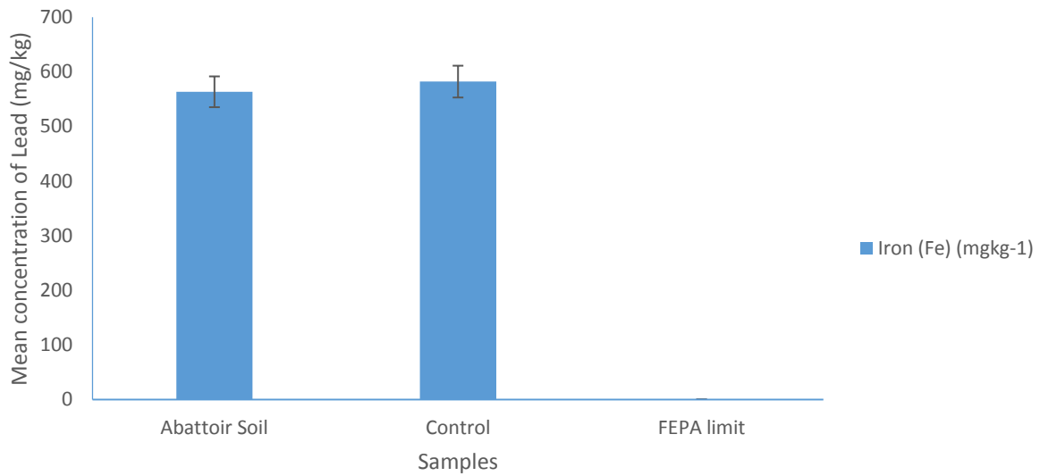
Fig. 4: concentration of Iron in the soil samples
