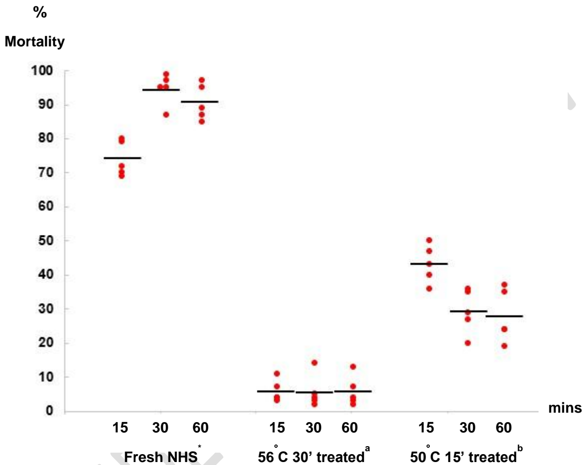
Fig. 1: Percentage of parasite mortality rate incubated with undiluted fresh normal human sera, heat-treated sera (56 °C 30 min) and (50 °C 15 min) against L. martiniquensis promastigotes at the different time intervals of 15, 30, and 60 mins
