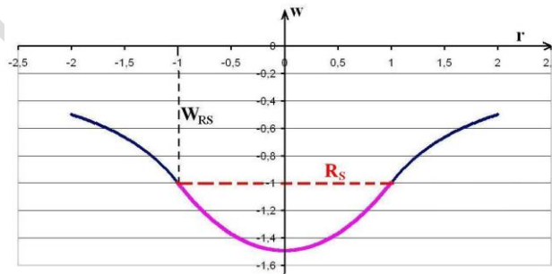
Fig. 4: Shape of the gravitational funnel
