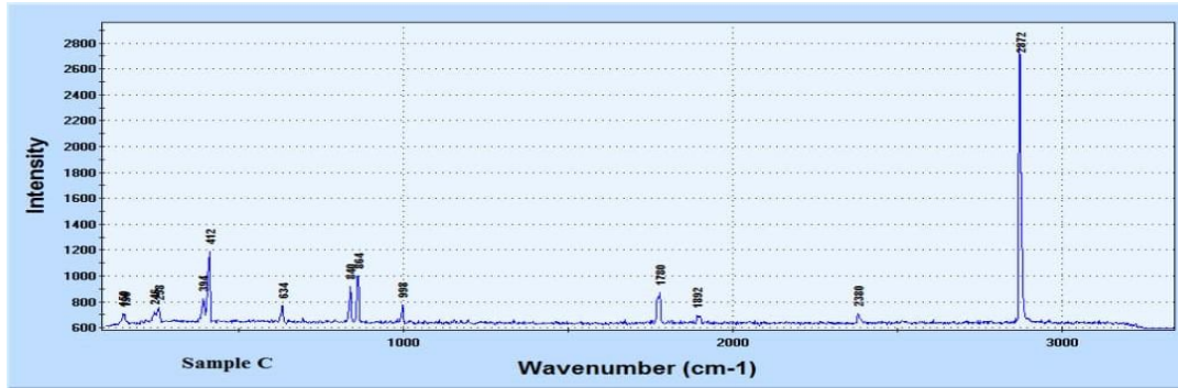
Fig. 1. The Raman Spectroscopic graphical result of Poly-O-Phenylenediamine doped at various percentage of silicon dioxide (a) 80% of Poly-O-Phenylenediamine to 20% of Silicon dioxide for sample A (b) 50% of Poly-O-Phenylenediamine to 50% of Silicon dioxide for sample B (c) 40% of Poly-O-Phenylenediamine to 60% of Silicon dioxide for sample C.
