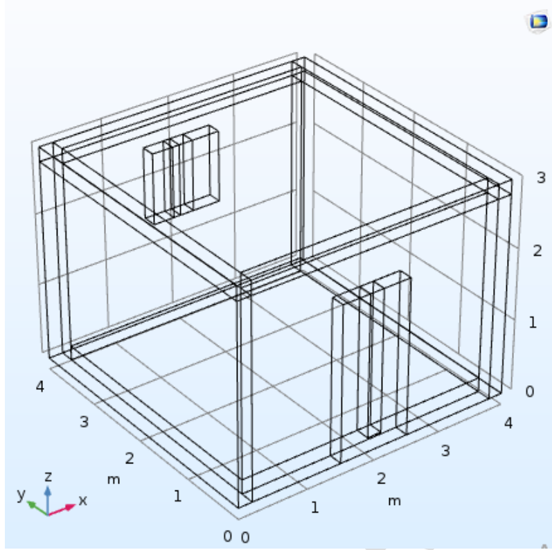
Figure 3: Building design model obtained with COMSOL Multiphysics 5.3a (source: author)
