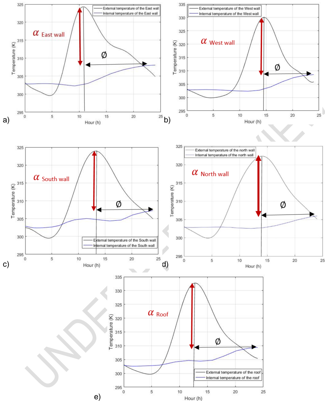
Figure 5: Evolution of temperatures of the inner and outer faces of walls, phase shift and thermal damping
