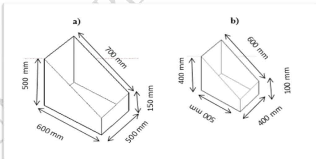
Figure 1: Dimensions of the box type solar cooker with an inclined surface; a) outer box and b) inner box [16].
