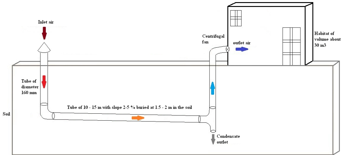
Fig. 1. Scheme of the system ASHE-habitat
