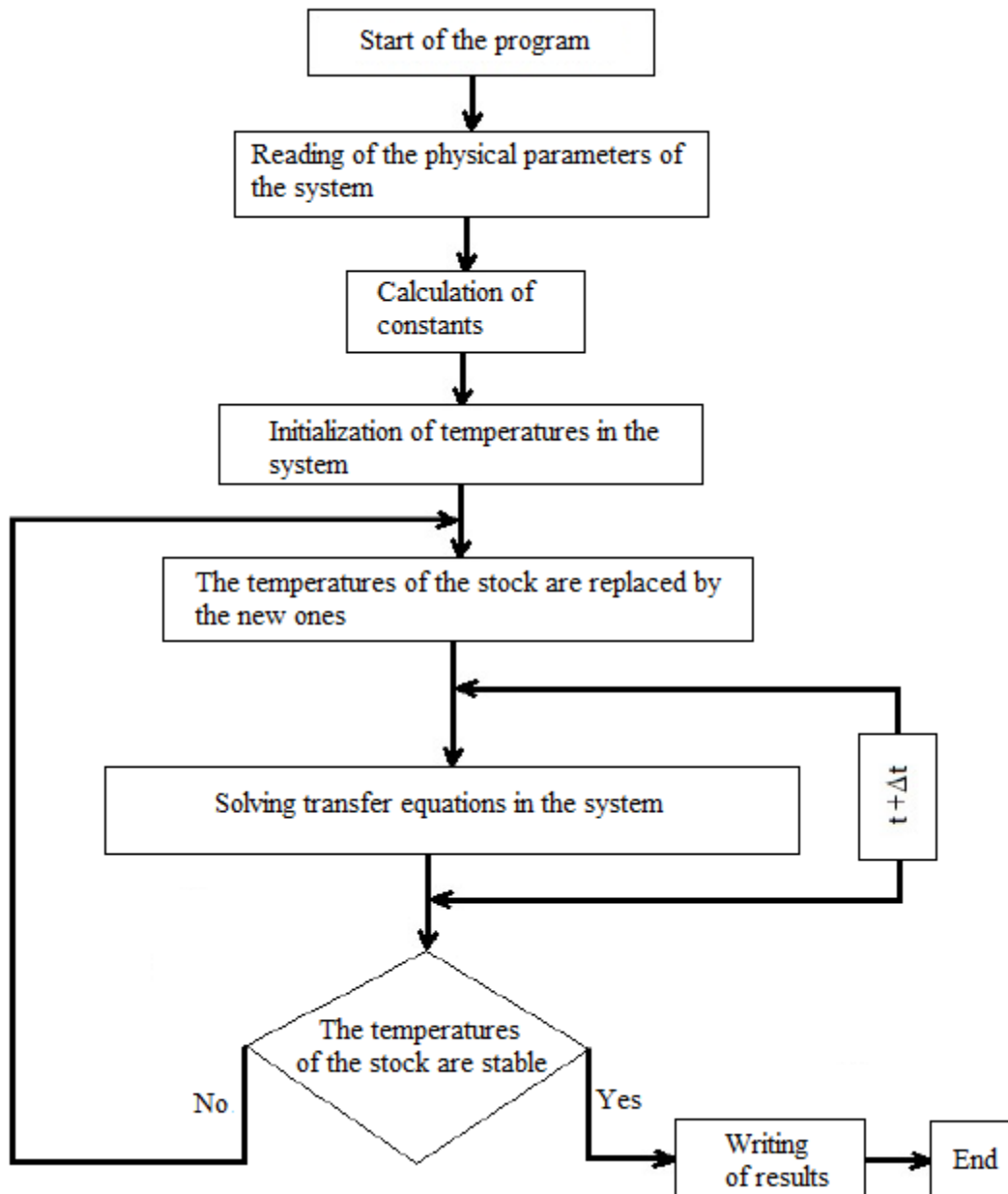
Fig. 3. Algorithm of simulation program
