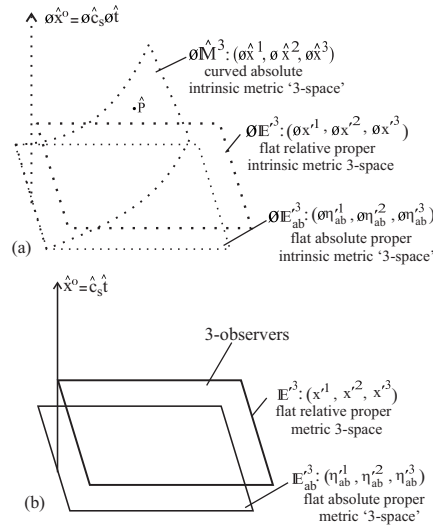
Figure 6: Figure 5 made more complete by including absolute proper metric ‘3-space’ \mathcal{E}_{ab}^3 as outward manifestation of \hat{\mathcal{O}}\hat{\mathcal{E}}_{ab}^3 in Fig.5 and the relative proper intrinsic metric 3-space \hat{\mathcal{O}}\hat{\mathcal{E}}^3 that underlies \mathcal{E}^3 in Fig.5.
