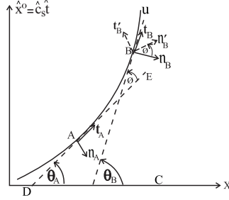
Figure 2: A one-dimensional metric space curving onto the absolute time ‘dimension’ along the vertical, projects a straight line one-dimensional metric space along the horizontal.
