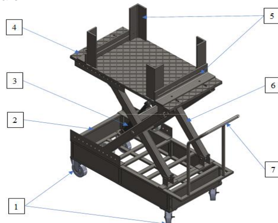
Figure 1: Overview of the lifting table
