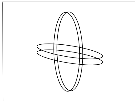
Fig.1 a representation of the quanton –anti quanton (Q+AQ) fields , note here that the radius of the quanton denotes only the decaying manner of the field intensity and does not outline the quanton physical domain
