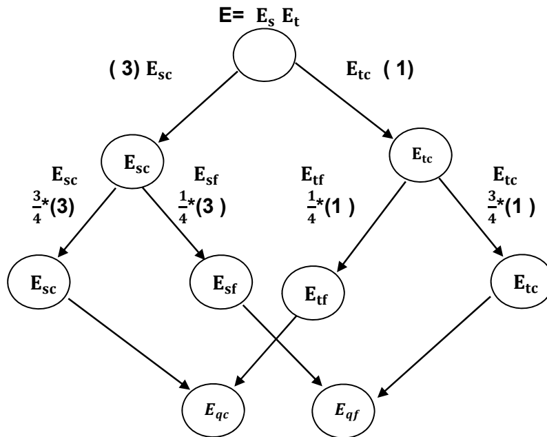
Fig.7. hypothetical tree diagram for the evolution and the degrees of freedom of anti quanton energy fields, and why the independent evolution of the anti quanton seems to be problematic in an inflationary scenario
