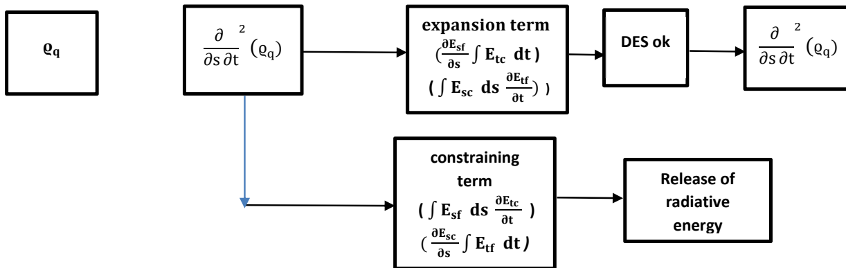
Fig. 4. Quanton energy density expansion process
