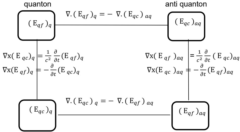
Fig.8 Maxwell equations fully define the space and time-varying fields of both quanton and anti quanton
