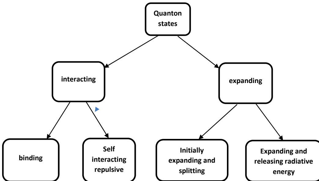
Fig.2. summary of the quanton states
