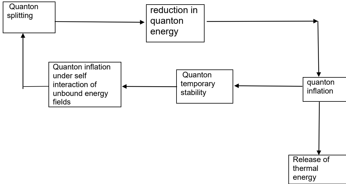
Fig. 5. cycle of quanton splitting and subsequent inflation
