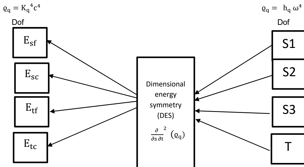
Fig. 3. role of dimensional energy symmetry in ensuring the uniformity of energy density distribution
