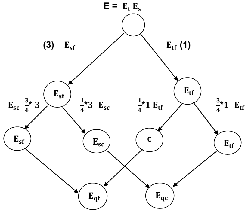
Fig.6. tree diagram for the evolution of the degrees of freedom of quanton's energy fields
