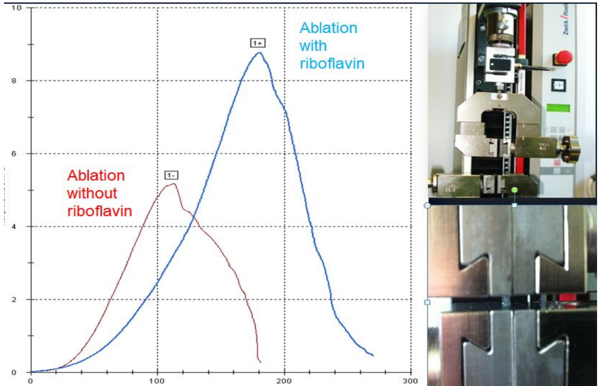
Fig. 1. Curves of biomechanical testing of thinned cornea samples after photoablation (without and with riboflavin). The vertical Y-axis is tension in MPa. The horizontal X-axis is elongation in %. Tensiometric device Zwick / Roell BZ 2.5 / TN1S (Germany) and a corneal-scleral flap installed in the clamps.
