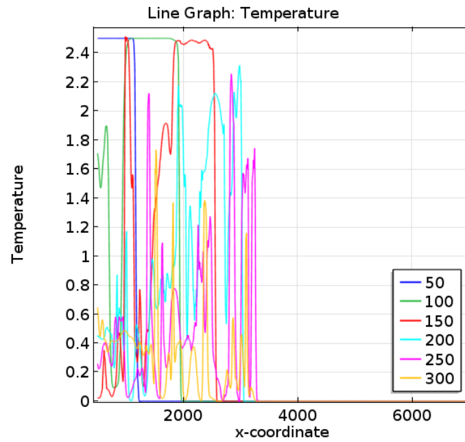
Fig. 13: Dimensionless temperature profiles at some point close to the surface \phi(X, 900) at time \tau = 50, 100, 150, 200, 250, 300 for plumes with Re = 500 , Pr = 7 , \phi_{in} = 2.5 and for Fr = 1
