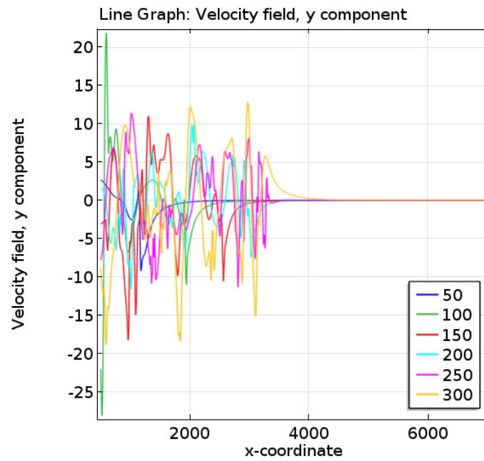
Fig. 14: Dimensionless vertical velocity profiles at some point close to the surface V(X, 900) at time \tau = 50, 100, 150, 200, 250, 300 for plumes with Re = 500 , Pr = 7 , \phi_{in} = 2.5 and for Fr = 1
