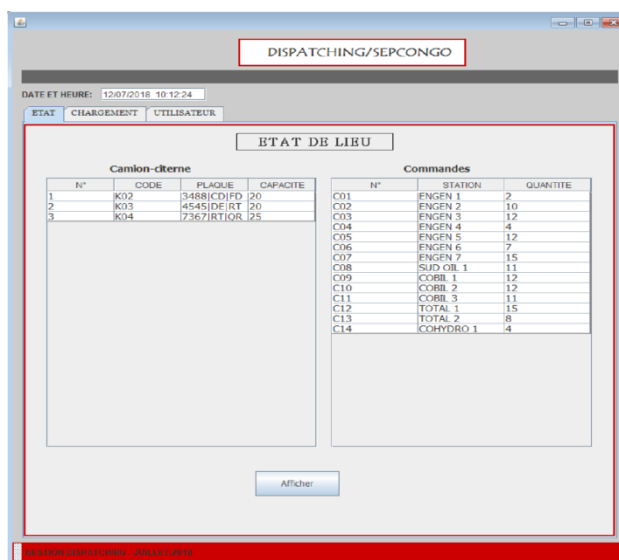
Fig 6: Main window.
