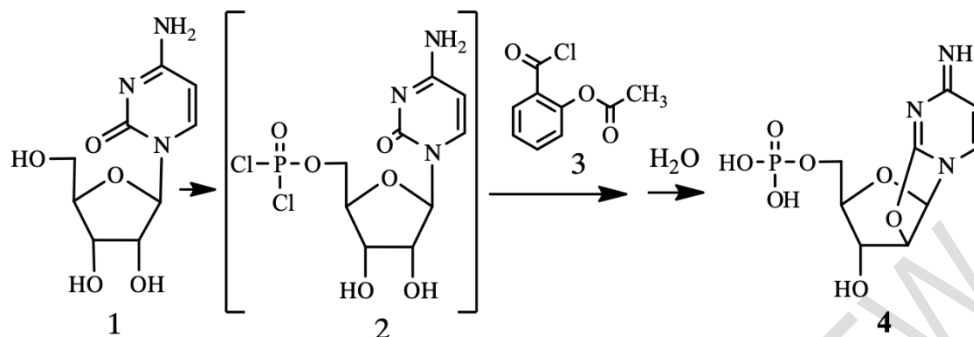
Fig. 4. Scheme of synthesis of cyclocytidine-5'-monophosphate
