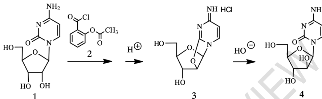
Fig. 1. Scheme of synthesis of arabinofuranosylcytosine
