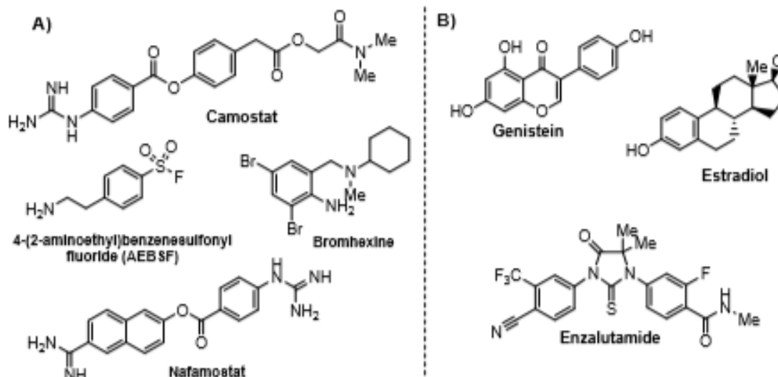
TMPRSS2 modulators. A) Chemical structure of TMPRSS2 inhibitors. B) Some transcriptional inhibitors of TMPRSS2
