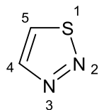
1,2,5-thiadiazole 1,2,4-thiadiazole 1,2,3-thiadiazole 1,3,4-thiadiazole
