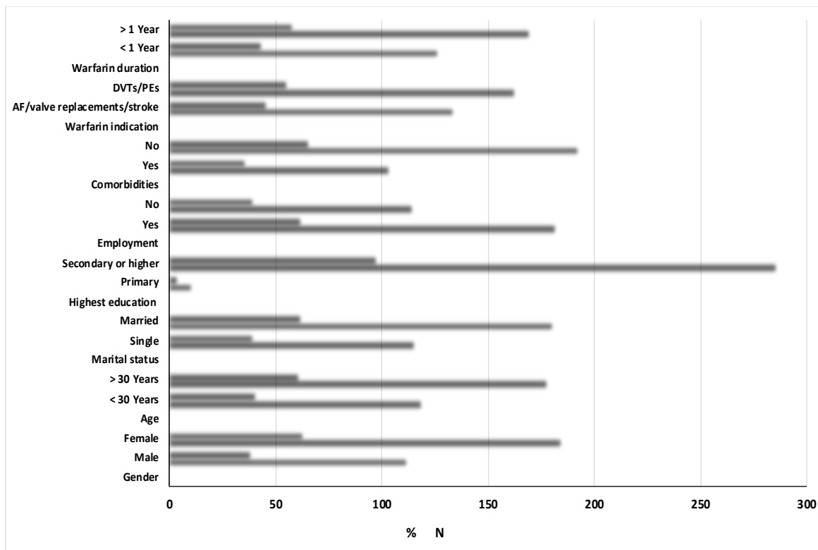
Figure 1: Demographic details of the warfarin patients
