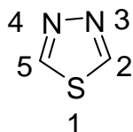
Fig. 2. Numbering of 1,3,4-thiadiazole ring system
