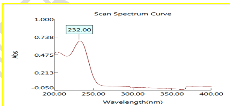
Figure 2: Determination of \lambda_{\max} of Metformin
