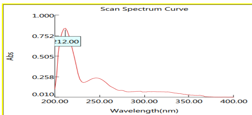
Figure 3: Determination of \lambda_{\max} of Sexagliptin
