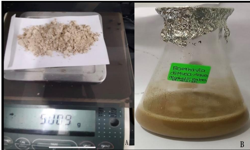
Figure 1 Schematic representation of Preparation of Boerhavia diffusa extract. A-powdered extract of Boerhavia diffusa . B-Aqua Alcoholic extract of Boerhavia diffusa .
