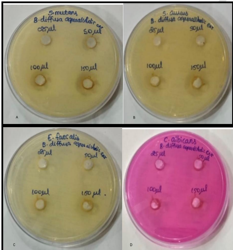
Figure 2 Anti-microbial activity of B. diffusa extract on A - Streptococcus mutans , B - Staphylococcus aureus , C - Enterococcus faecalis , and D - Candida albicans
