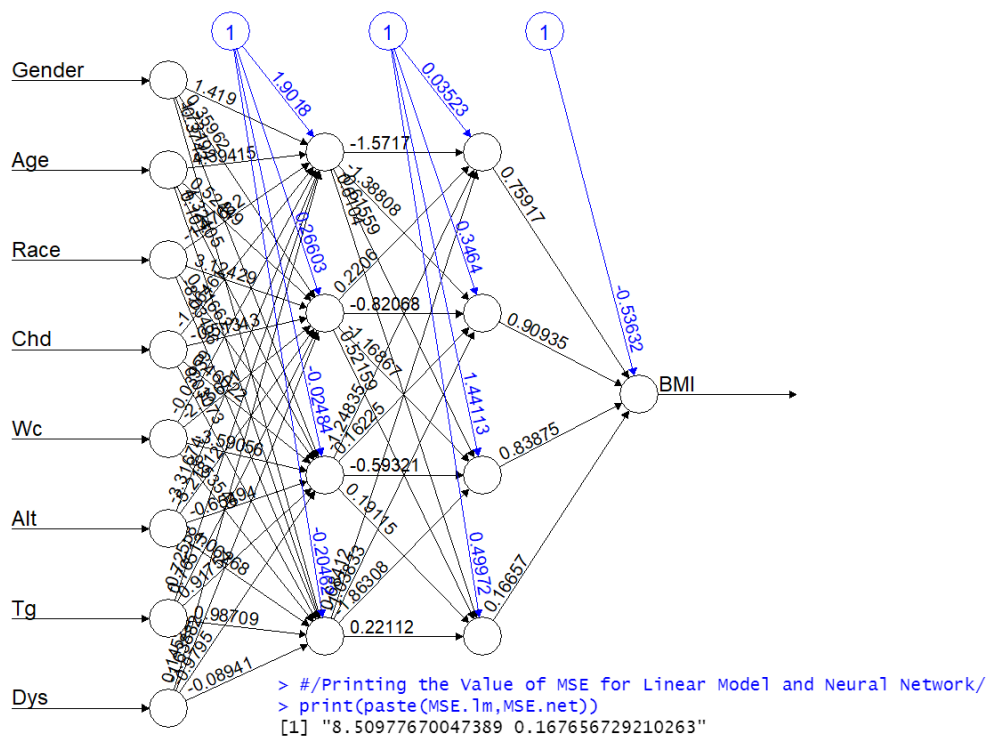
Figure 2. The architecture of the best (MLP) model with eight input variables, two hidden layers, and one output node (Proposed Model)
