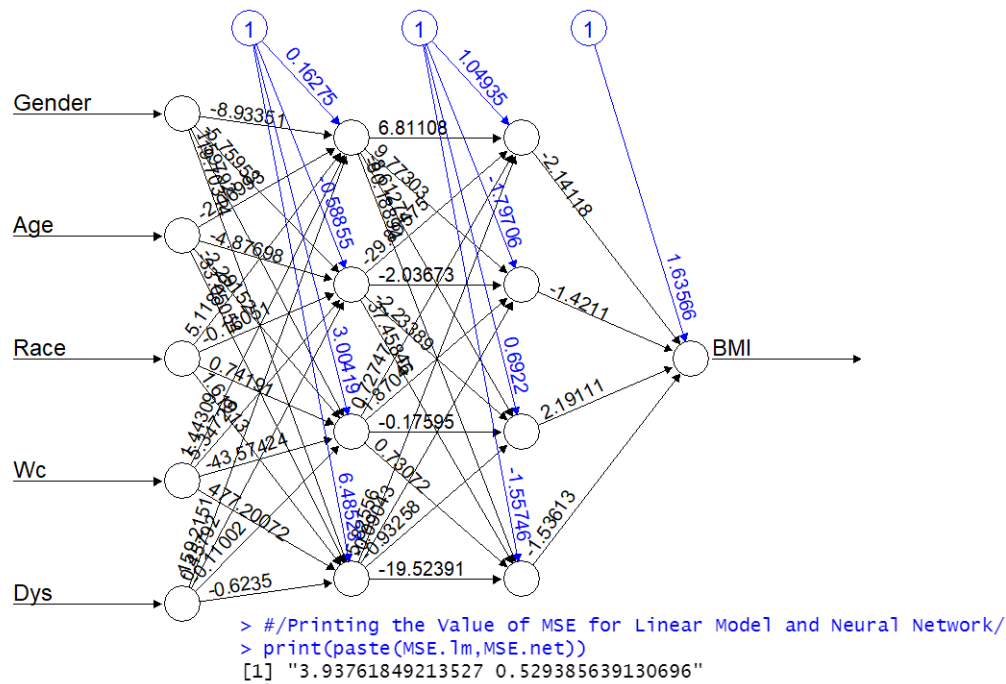
Figure 4. The architecture of the best (M.L.P.) model with five input variables, two hidden layers, and one output node
