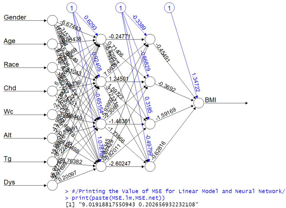
Figure 3. The architecture of the best (MLP) model with eight input variables, two hidden layers, and one output node
