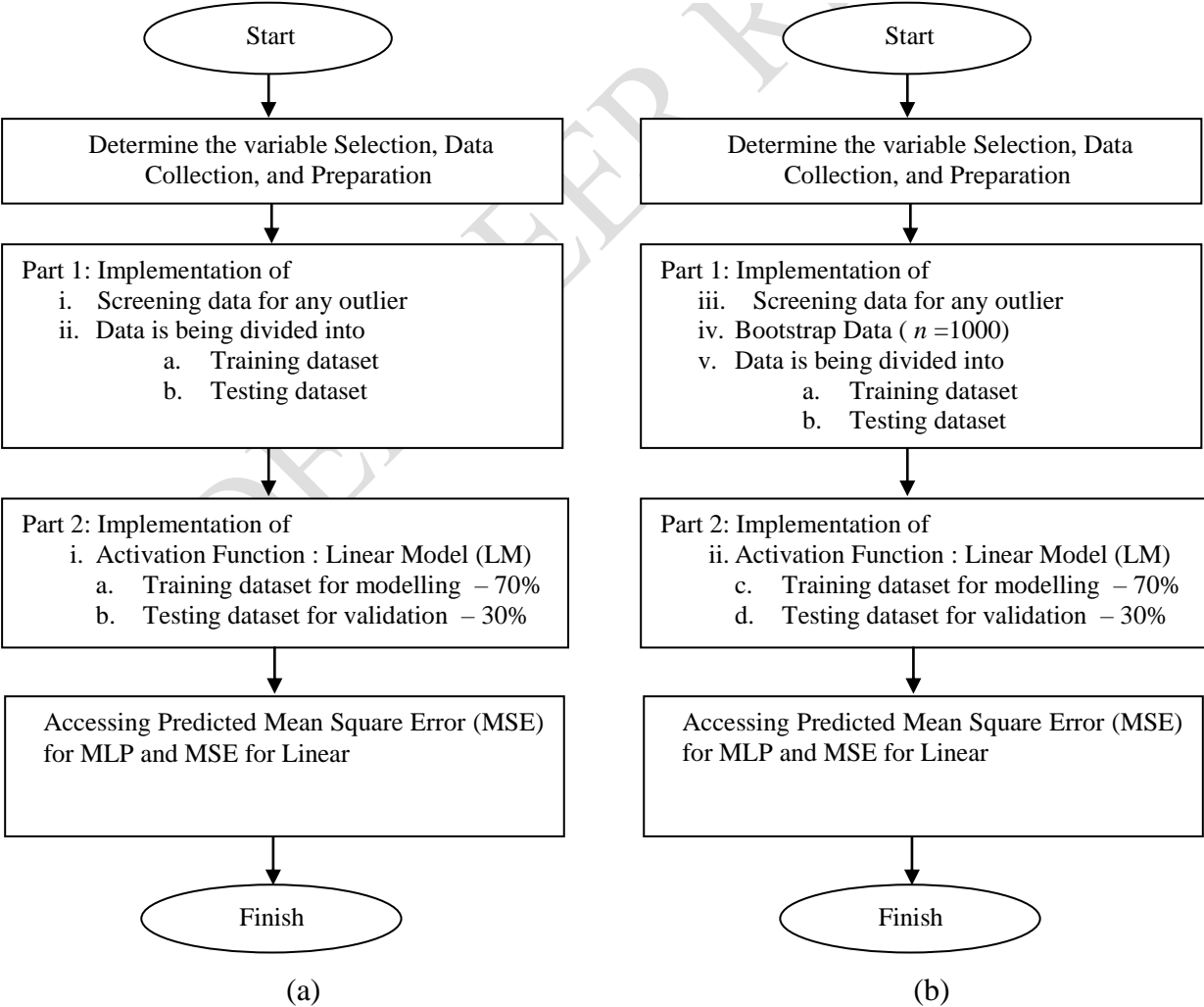
Figure 1. Flowchart illustrating the proposed statistical linear modelling technique
