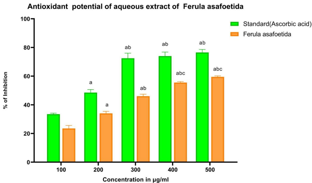
Figure 1: The figure represents the antioxidant potential of aqueous extract of Ferula asafoetida by DPPH assay. The X axis represents the concentration in ug/ml and the Y axis represents the % of inhibition. Green bar represents ascorbic acid, orange bar represents aqueous extract of Ferula asafoetida . Each bar represents the Mean±SEM of 3 independent observations. Significance at p < 0.05 .
