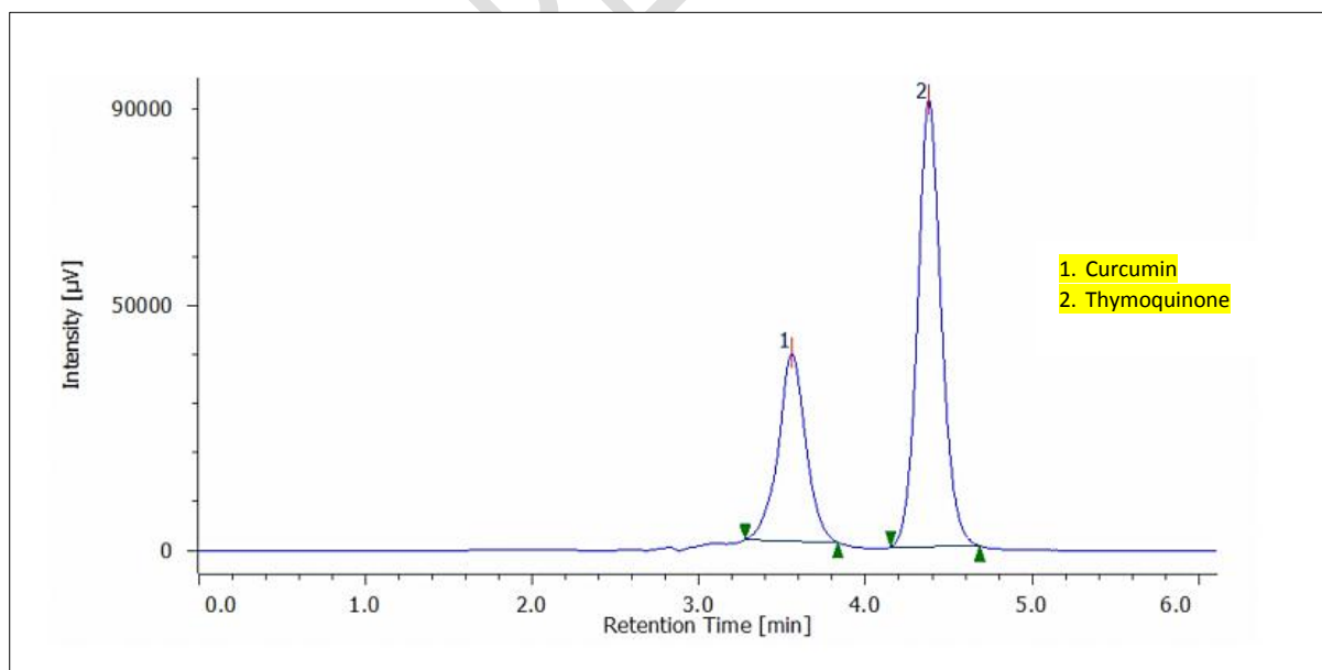
Fig3. Chromatogram of Curcumin and Thymoquinone obtained from the sample solution
