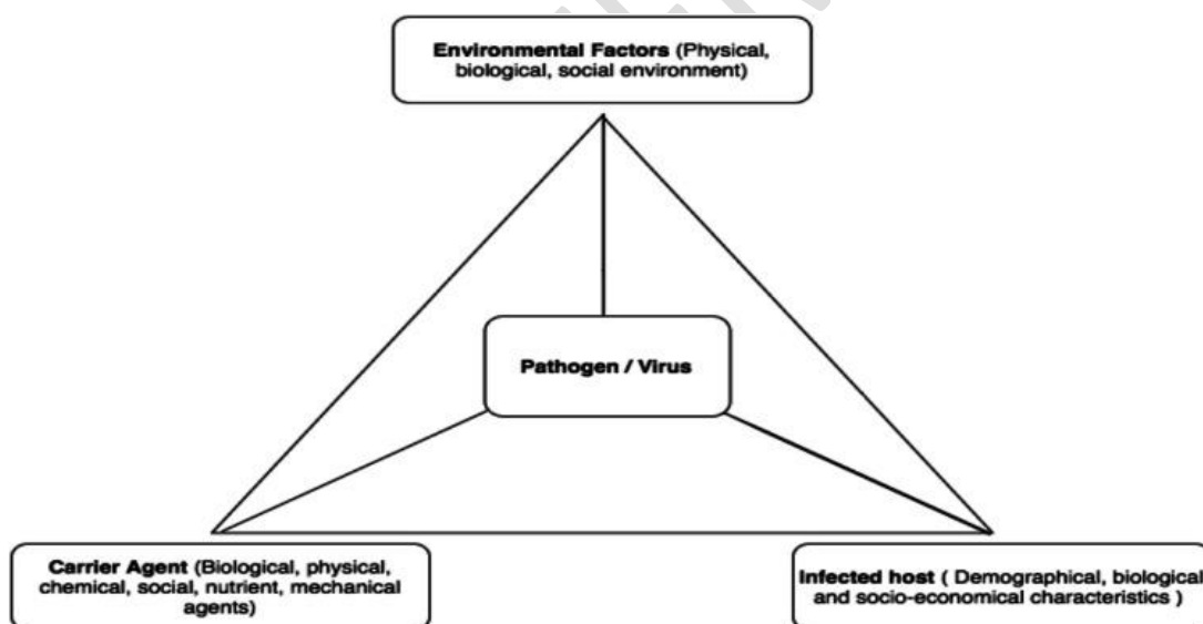
Fig. 2. Environmental factors
