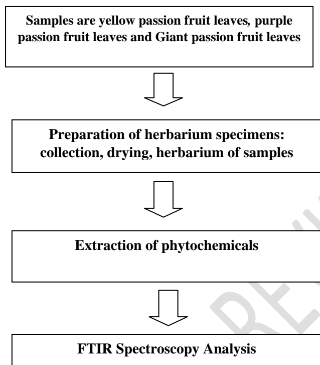
Figure :1. Flowchart of FTIR Spectroscopy analysis process.
