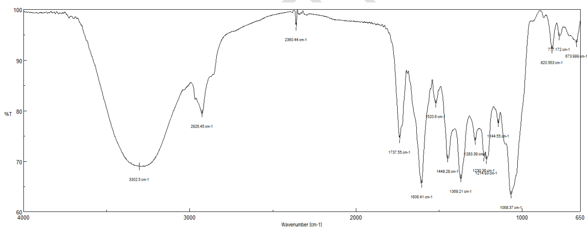
Figure 4 FTIR Spectra of Passiflora quadrangularis leaf
