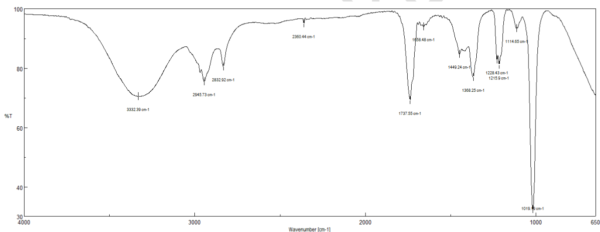
Figure 3 FTIR Spectra of Passiflora edulis leaf
