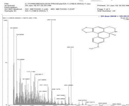
II-c (Mass spectral data)
