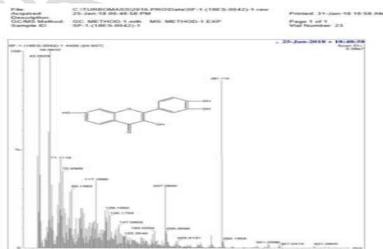
III-c (Mass spectral data)
