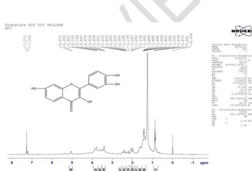
III-b( 1 H-NMR spectral data)
