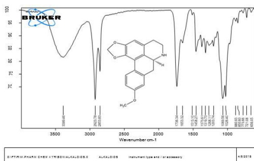
Fig 2: Spectral data of compound II II-a (IR spectral data)
