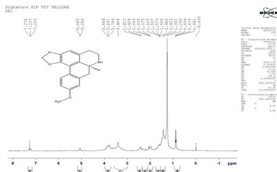
II-b ( 1 H-NMR spectral data)
