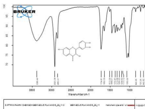
III-a (IR spectral data)
