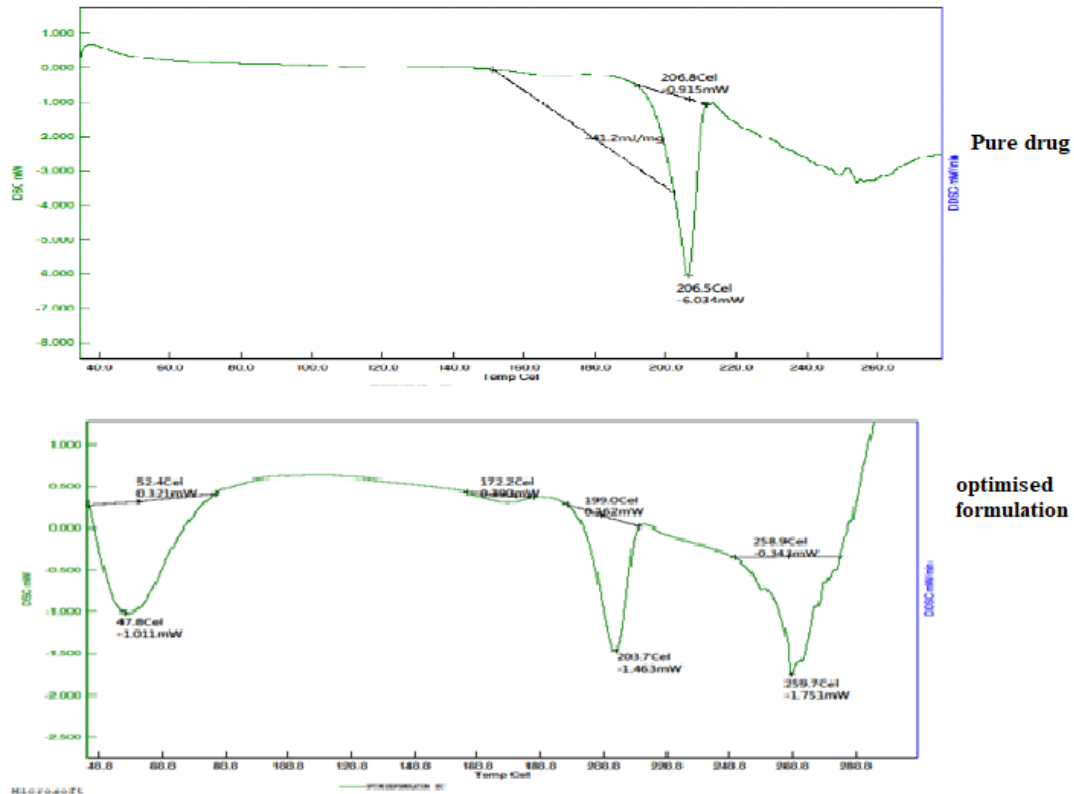
Figure 2: DSC studies of a pure drug (Fexofenadine HCl) & Optimized formulation (G1)
