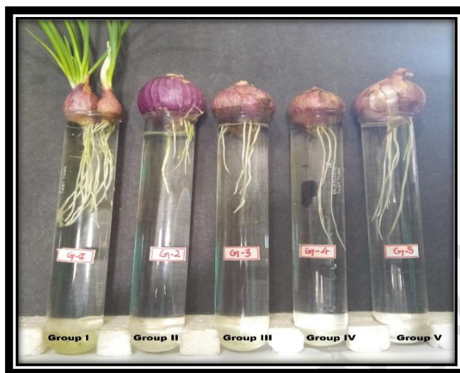
Figure 4 Genoprotective activity of Indigofera tinctoria leaves extract in experimental step up
