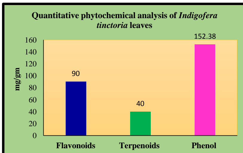
Figure 1 Quantitative phytochemical analysis of Indigofera tinctoria leaves powder
