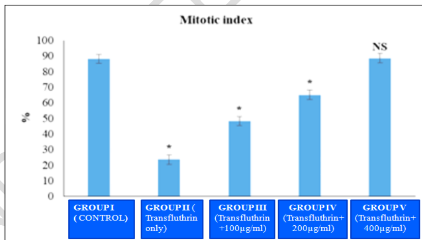
Figure 5 Effect of Indigofera tinctoria leaves on mitotic index of Allium cepa root
