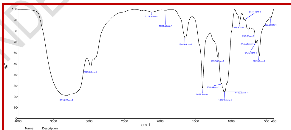
Figure 2 FTIR peak of Indigofera tinctoria
