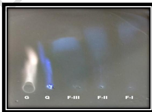
Figure 3 Identification of the phenolic compound using Column chromatography eluting and TLC from Indigofera tinctoria leaves extract
