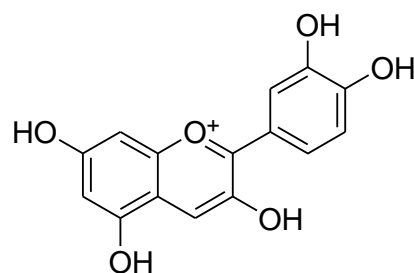
Fig 2: Cyanidin
