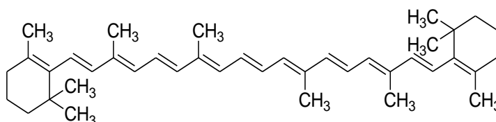
Fig 3 \beta - carotene
