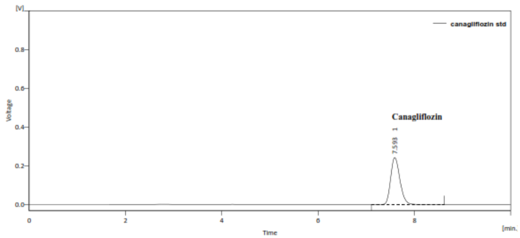
Figure-6: Chromatogram of Canagliflozin Individual Standard Solution:
