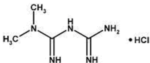
Figure-2: Chemical Structure of Metformin HCl
