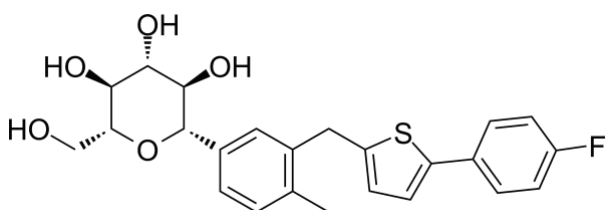
Figure-1: Chemical Structure of Canagliflozin
