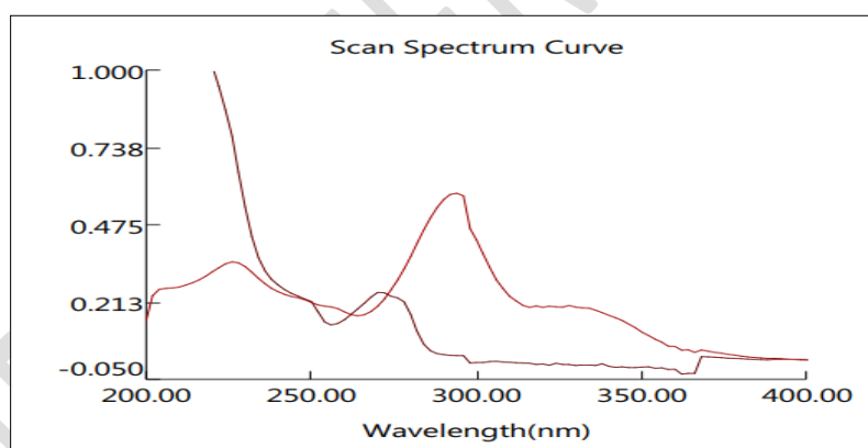
Fig. 4: overlay spectra of EMPA and LINA
