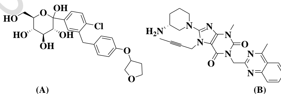
Fig. 1: Chemical structure of (A) Empagliflozin and (B) Linagliptin
