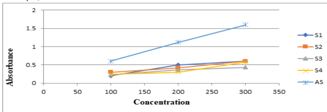
Figure 4. Phosphomolybdate Assay
