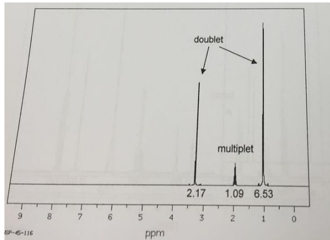
Graph: 1 Spectrum of oleic acid
