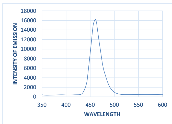
Fig. 10. The emission profile of common blue LED
