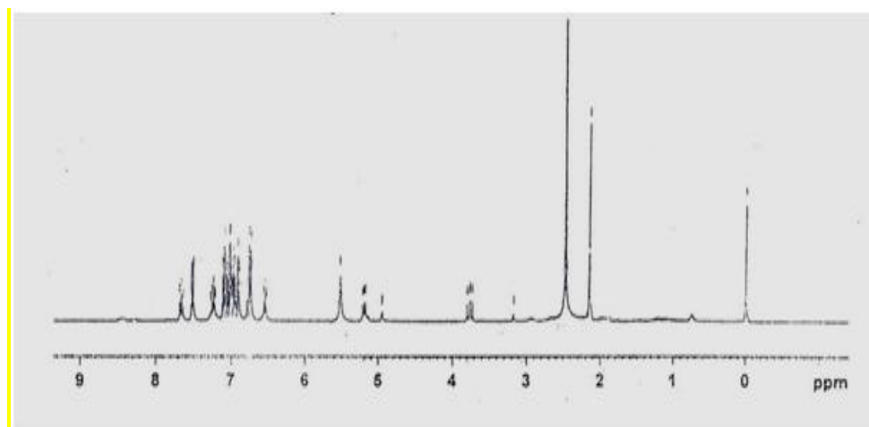
Figure 2: 1NMR spectra of compound A8
