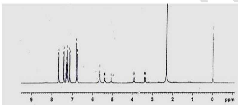
Fig. 1: ^1H NMR spectra of compound C2
