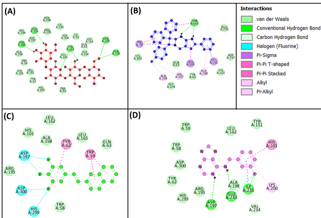
Figure 2. Molecular interactions analysis of best docked ligands with α-amylase (2QV4) enzyme. (A) Redocked acarbose; (B) C7 compound; (C) C4 compound; (D) C3 compound.
