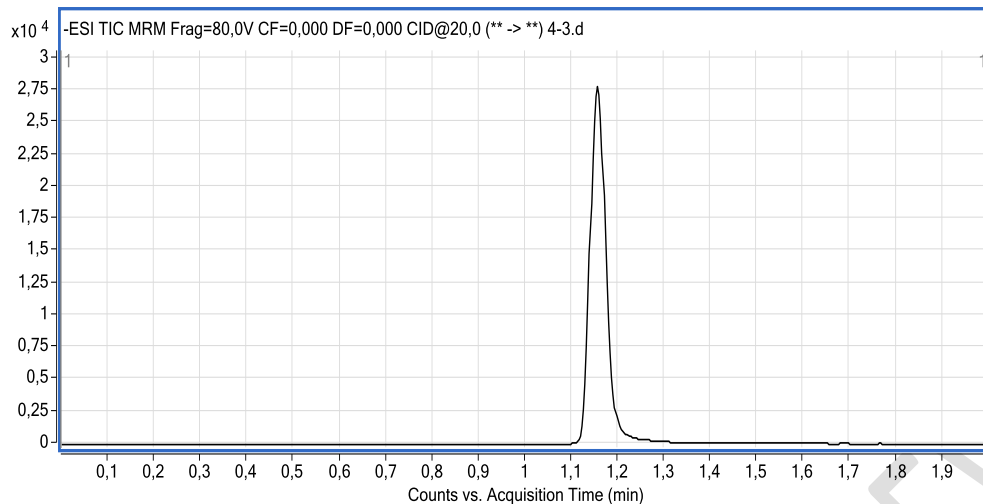
Fig. 7. Chromatogram (Sample solution, 4 \mu\text{g mL}^{-1} ).
