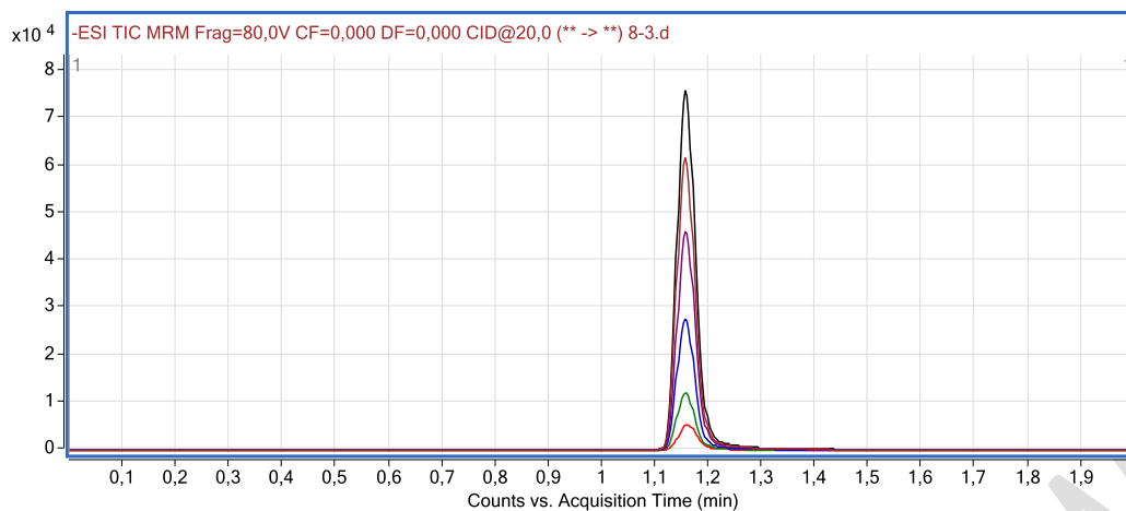
Fig. 4. Overlay chromatogram (Standard solutions, 1, 2, 4, 6, 8, 10 \mu\text{g mL}^{-1} )
