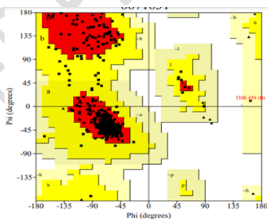
Fig. 6. Ramachandran plot obtained using PROCHECK
