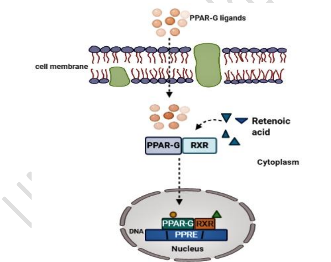
Fig 1. PPAR-G and RXR signalling on binding of ligand
