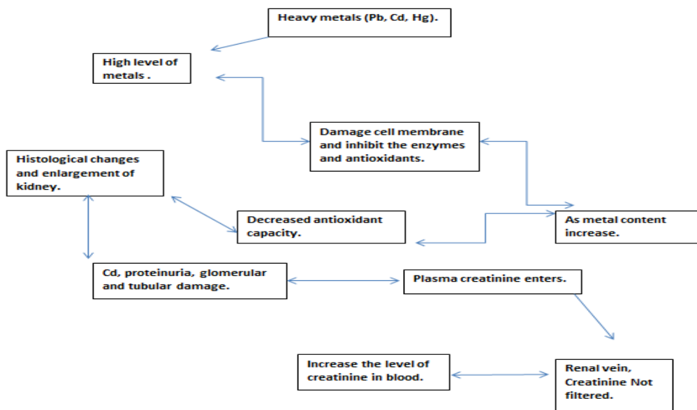
Figure 1: Shows the mechanism of increasing Creatinine level in blood.
