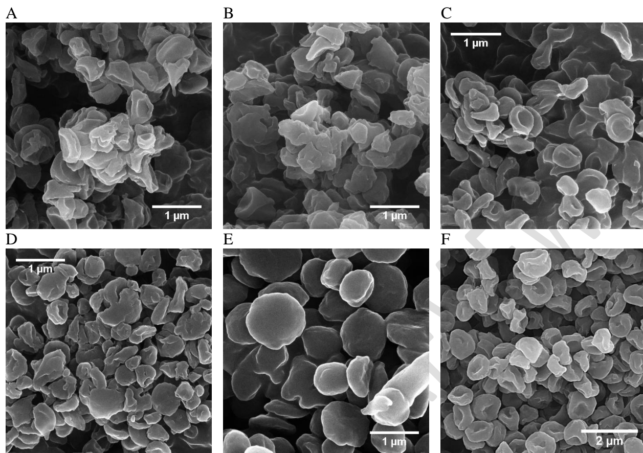
Fig. 2. FESEM images of GB-SP nanomicelles prepared with Act/Eth (A) \text{SPE}_3 & (B) \text{SPE}_{3/2} , Act/MeOH (C) \text{SPM}_2 & (D) \text{SPM}_{4/2} , and DCM/Eth (E) \text{EM}_4 & \text{EM}_{4/2} .
