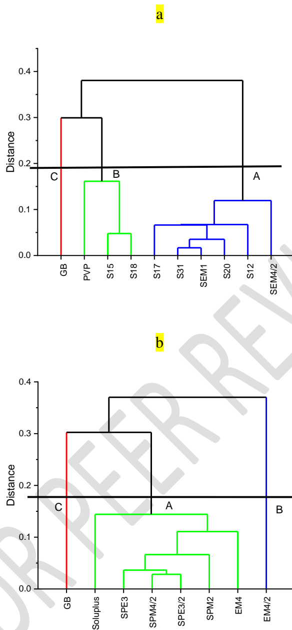
Fig. 5. Hierarchical Cluster Analysis (HCA) for FTIR Spectra of (a) GB-PVP nanoparticles and (b) GB-SP nanomicelles.
