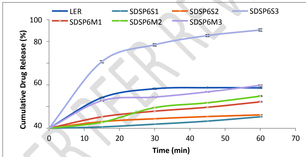
FIGURE 1 (d) Dissolution profile of Solid Dispersions prepared with PEG6000
