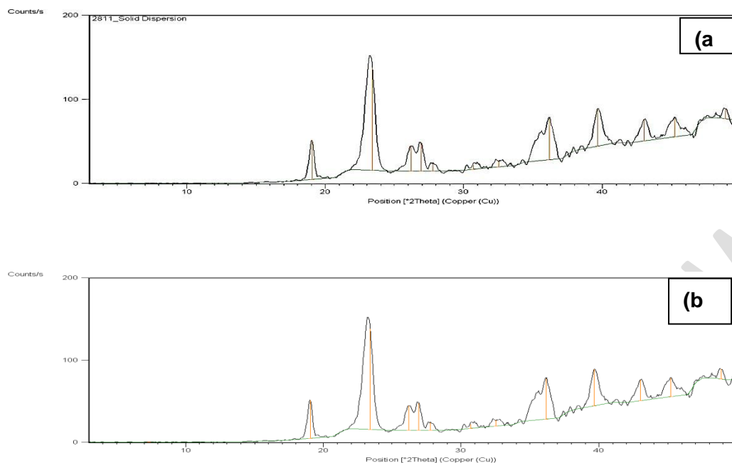
FIGURE 11 Powdered X Ray diffraction patterns of Optimized solid dispersion of LER and PEG6000 (a) at zero time (b) after storage of 6 months
