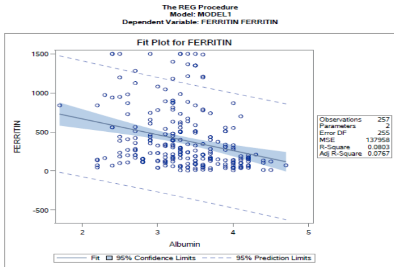
Figure :2 Shows the regression analysis of ferritin and albumin
