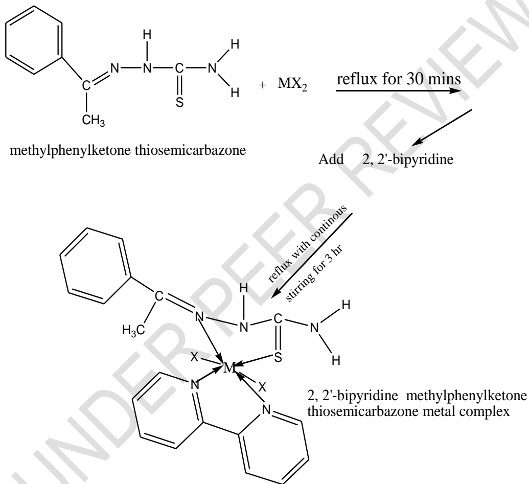
Scheme 2: Synthetic procedure of metal complex of methylphenylketone thiosemicarbazone with 2, 2'-bipyridine
