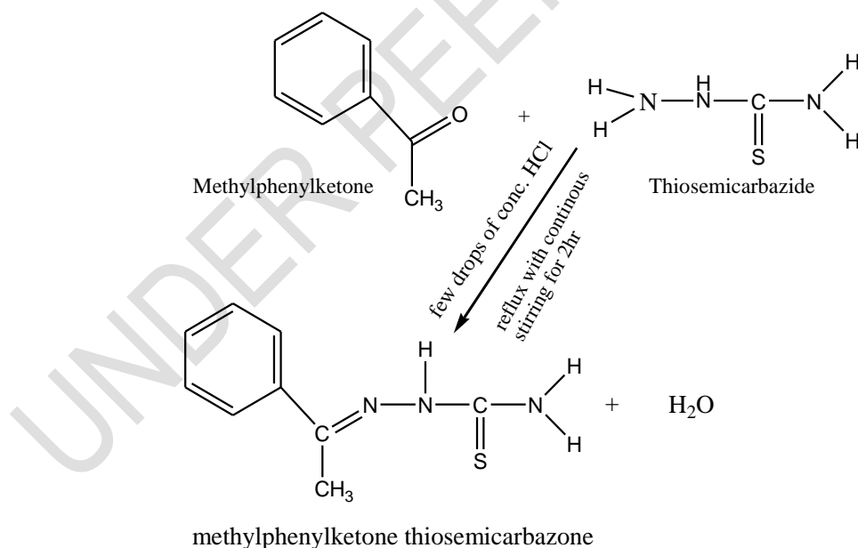
Scheme 1: Synthetic procedure of the ligand methylphenylketone thiosemicarbazone through condensation reaction
