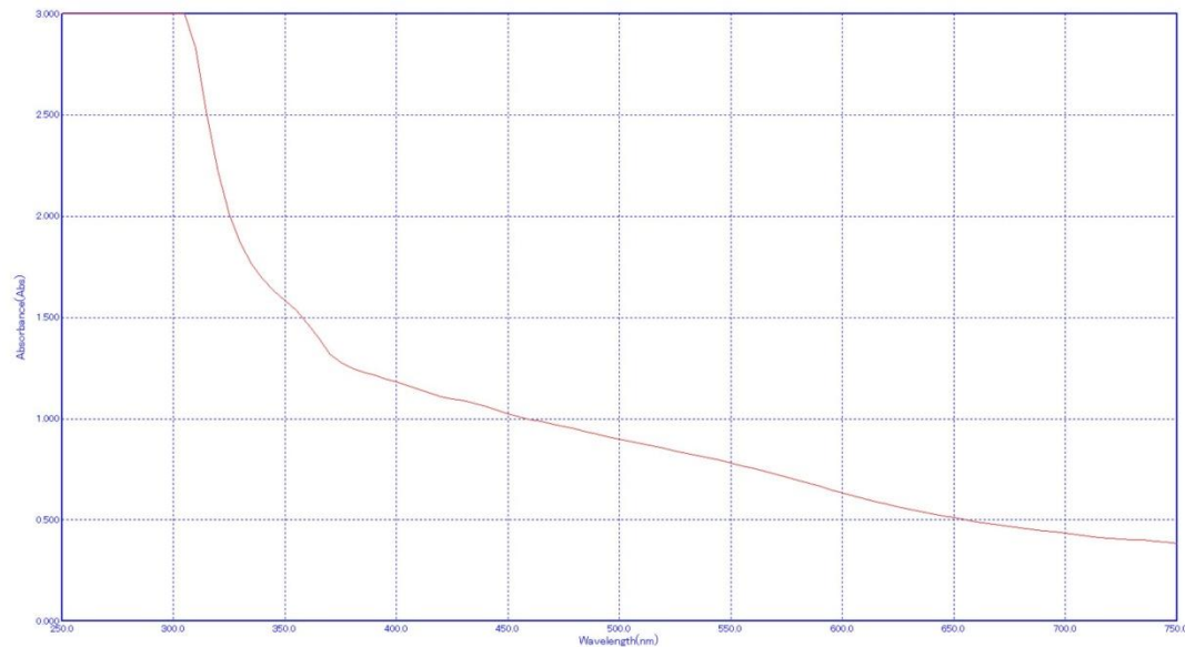
Figure 2 : UV Spectroscopy
