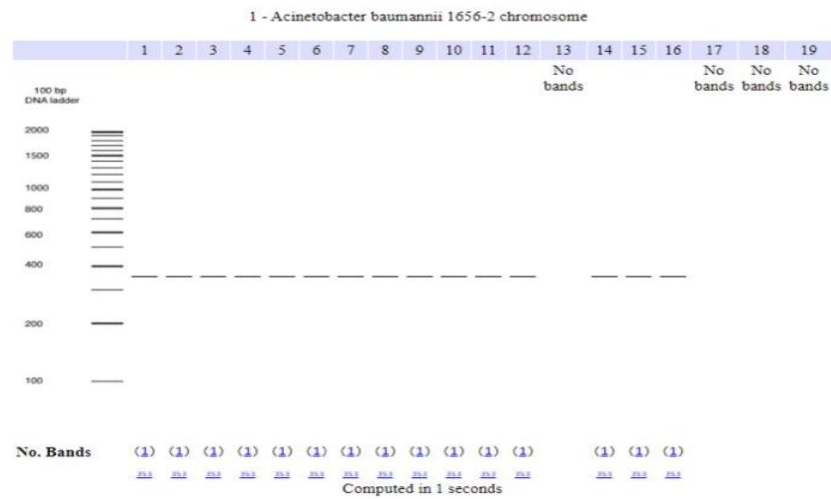
Figure 1 Amplification bands showing positive for blaOXA-51 like using in-silico PCR amplification among the strains of A. baumannii with an amplicon size of 353bp.
