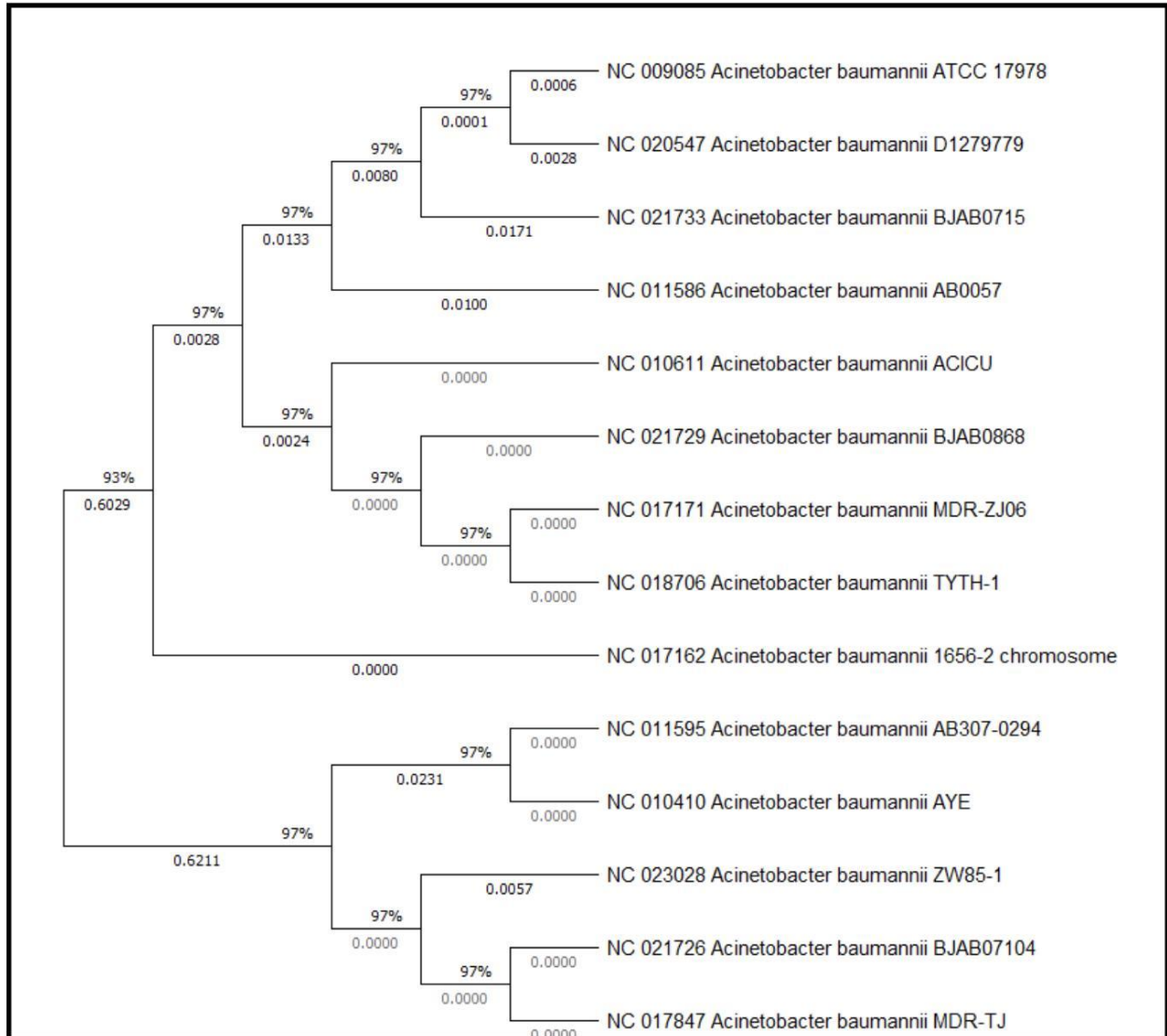
Figure 3: Phylogenetic tree construction for blaOXA-51like using in-silico PCR amplification among the strains of A. baumannii
