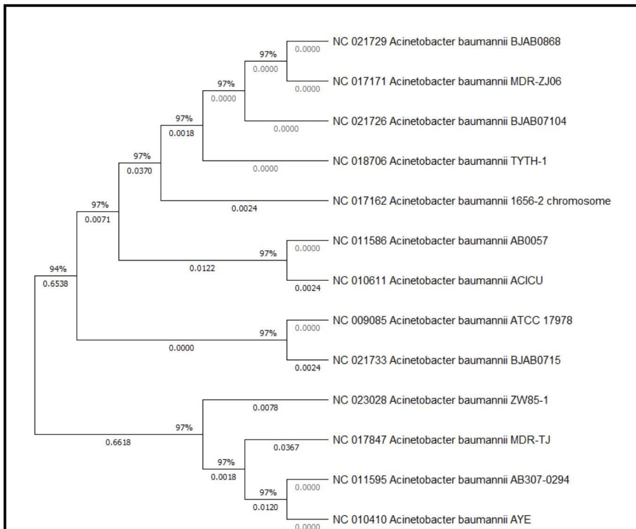
Figure 4: Phylogenetic tree construction for blaADC using in-silico PCR amplification among the strains of A. baumannii
