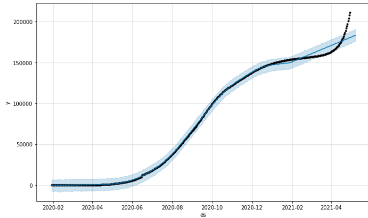
Fig. 3. Graph of Predicted total no. of death cases
