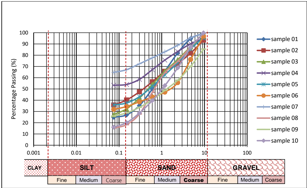
Figure 1 a: Sieve Analysis Test Result Sample 1 -10
