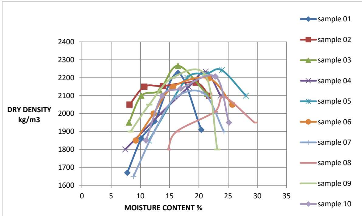
Figure 3a: COMPACTION TEST FOR SAMPLE 1- 10
