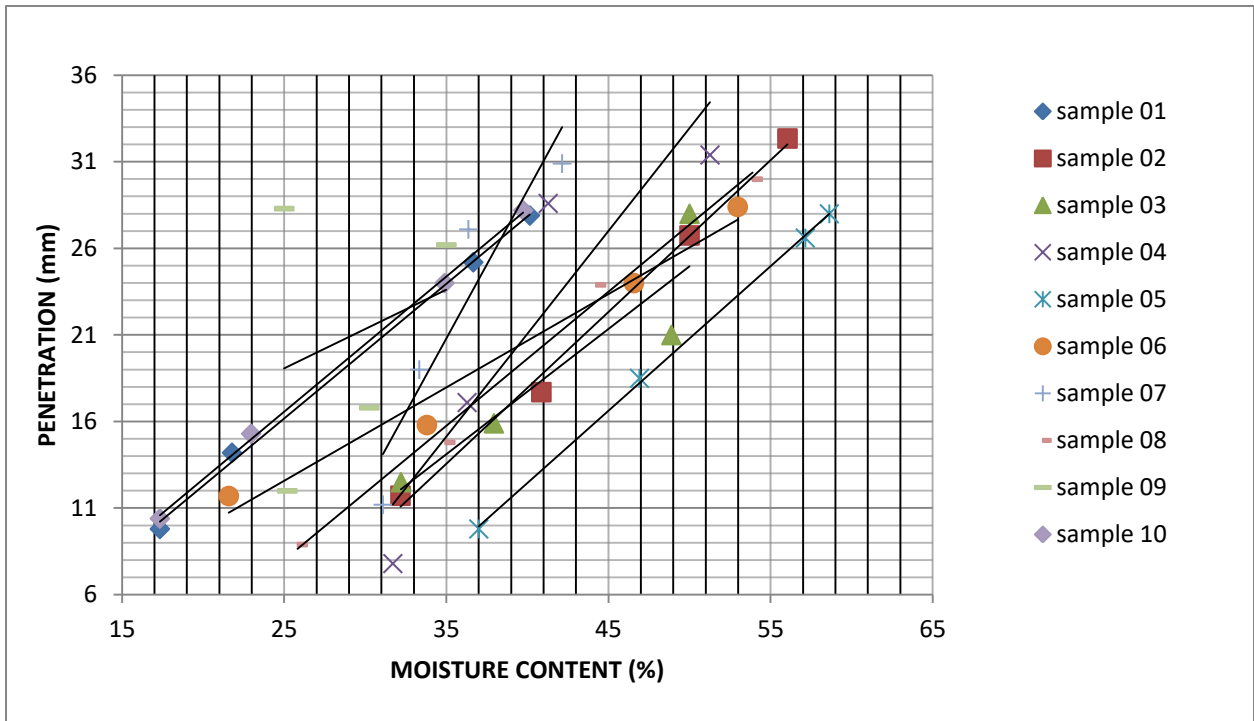
Figure 2 a: Liquid Limits Test Result Sample 1-10
