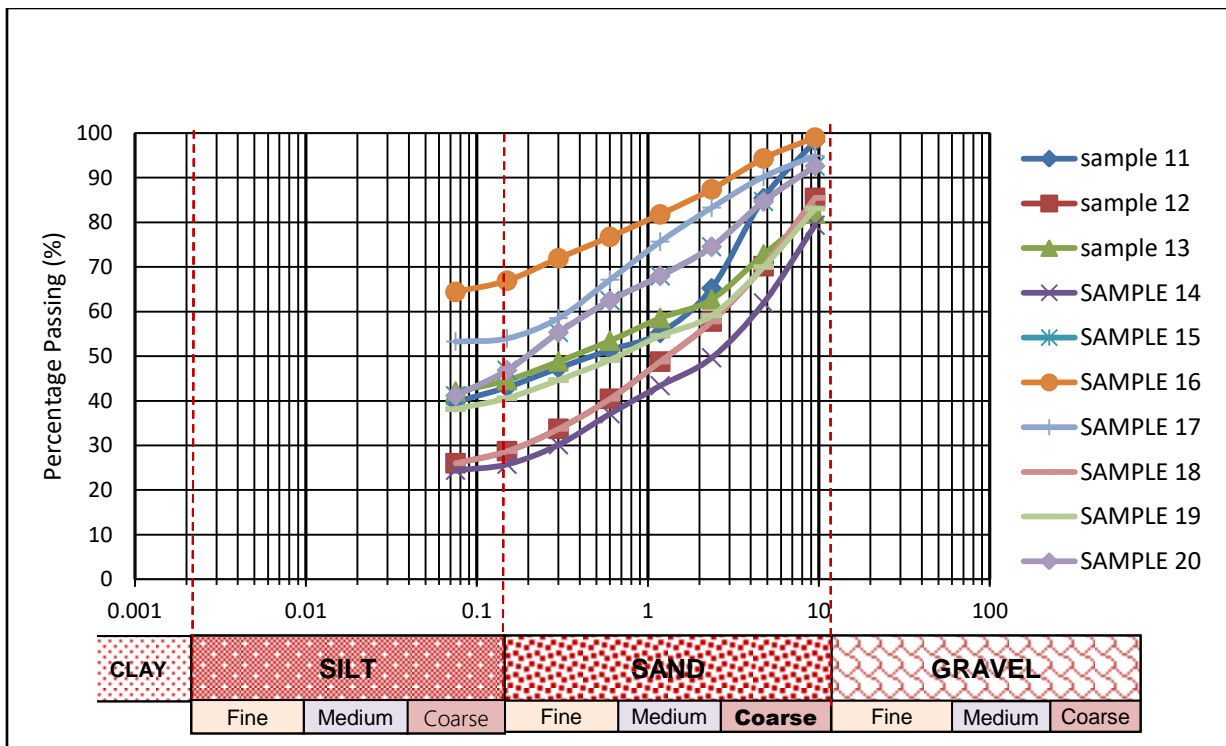
Figure 1b: Sieve Analysis Test Result Sample 11 -20
