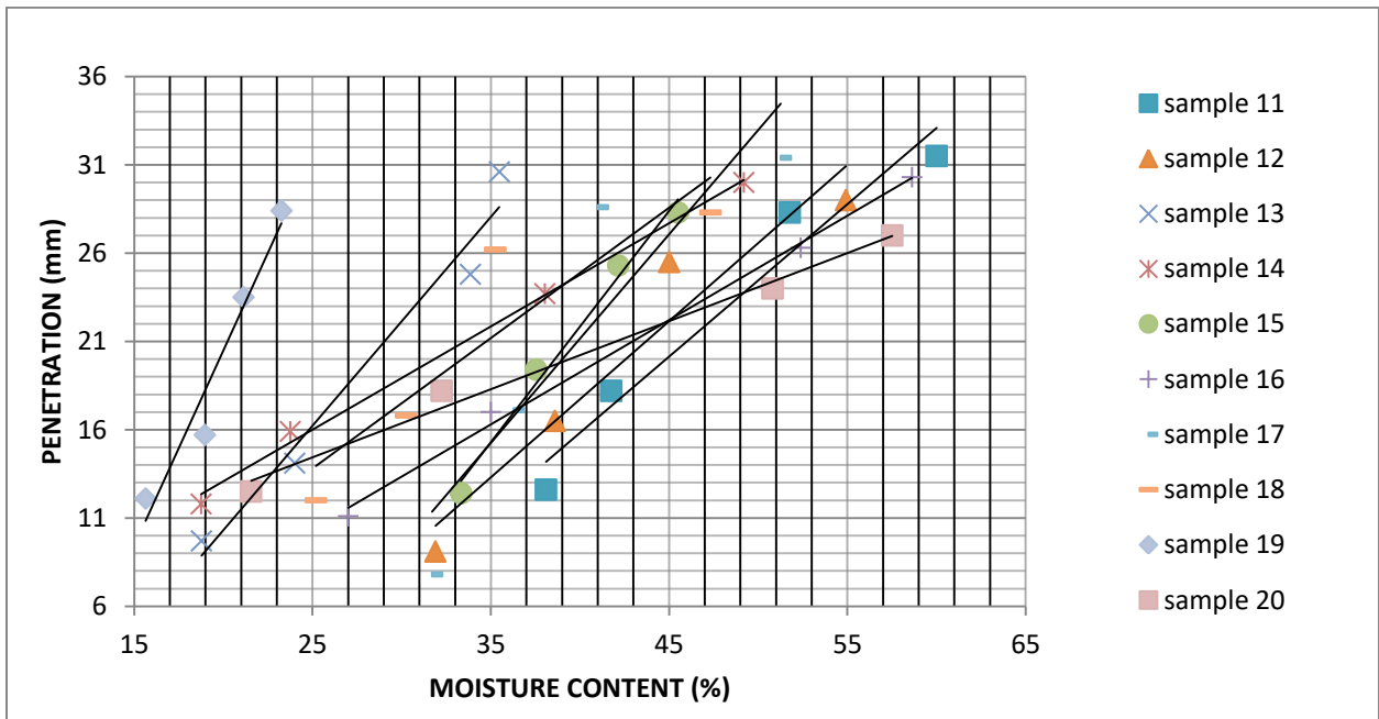
Figure 2 b : Liquid Limits Test Result Sample 11-20
