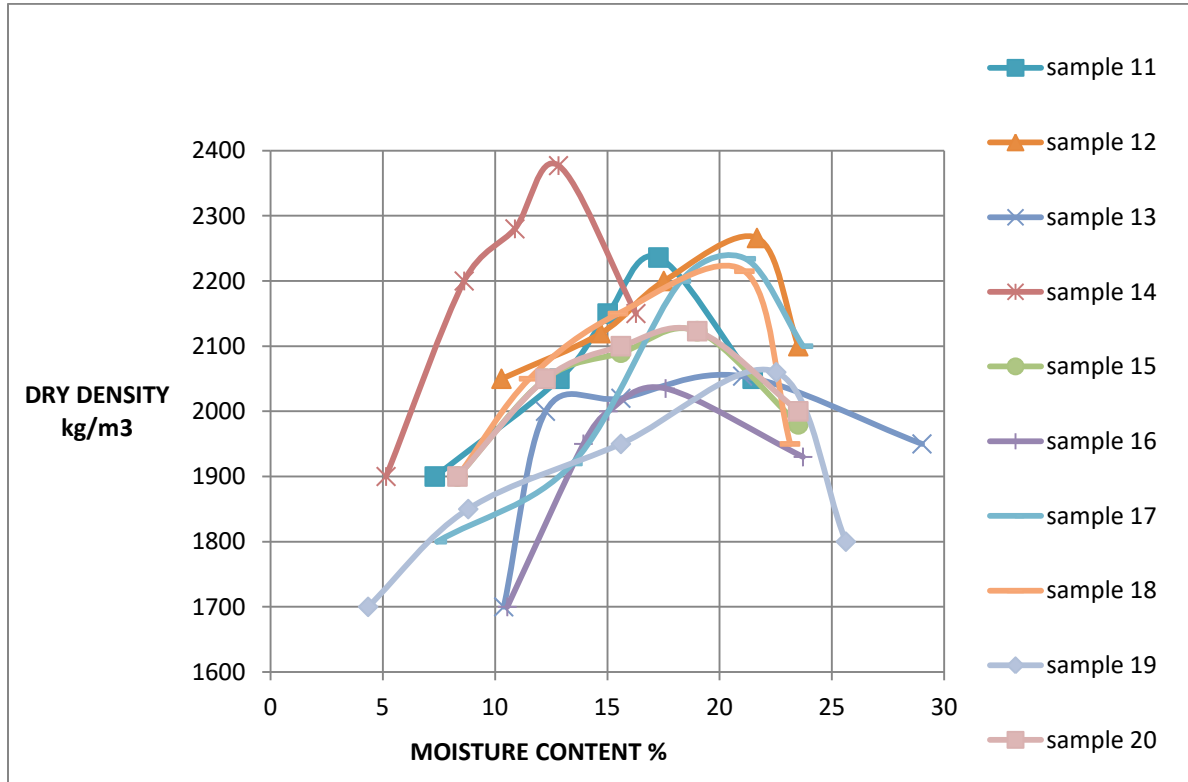
Figure 3 b : COMPACTION TEST FOR SAMPLE 11-20
