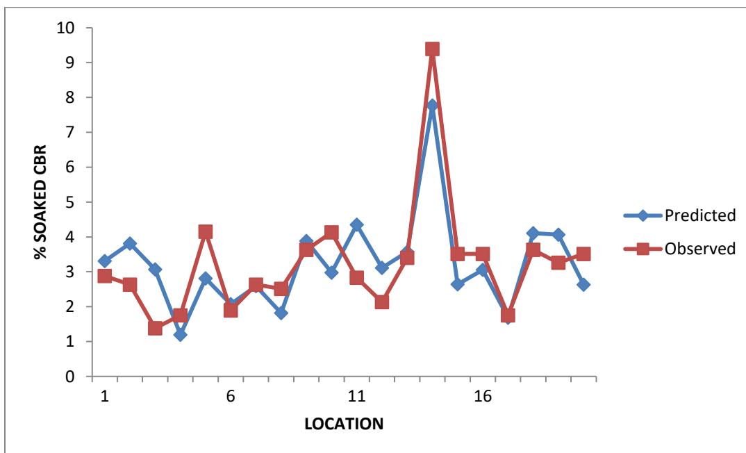
Fig.2. Graph of predicted against observed CBR
