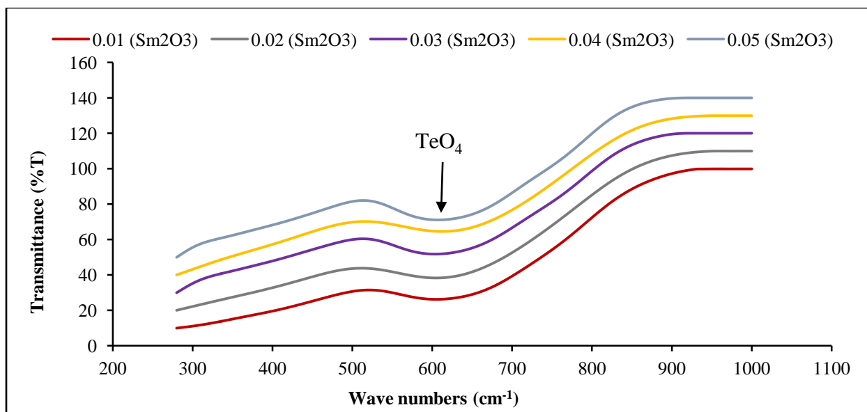
Figure 3: Plot of FTIR spectra for [(\text{TeO}_2)_{0.7} (\text{ZnO})_{0.3}]_{1-x} [\text{Sm}_2\text{O}_3]_x glasses.
