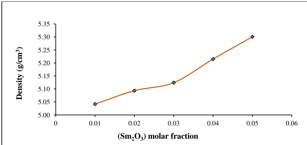
Figure 1: Plot of density for [(TeO 2 ) 0.7 (ZnO) 0.3 ] 1-x [Sm 2 O 3 ] x glasses.
