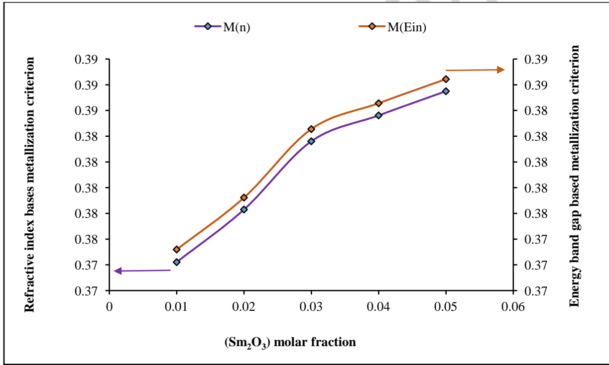
Figure 17: Metallization criterion based refractive index and band gap energy for [(\text{TeO}_2)_{0.7} (\text{ZnO})_{0.3}]_{1-x} [\text{Sm}_2\text{O}_3]_x glasses.
