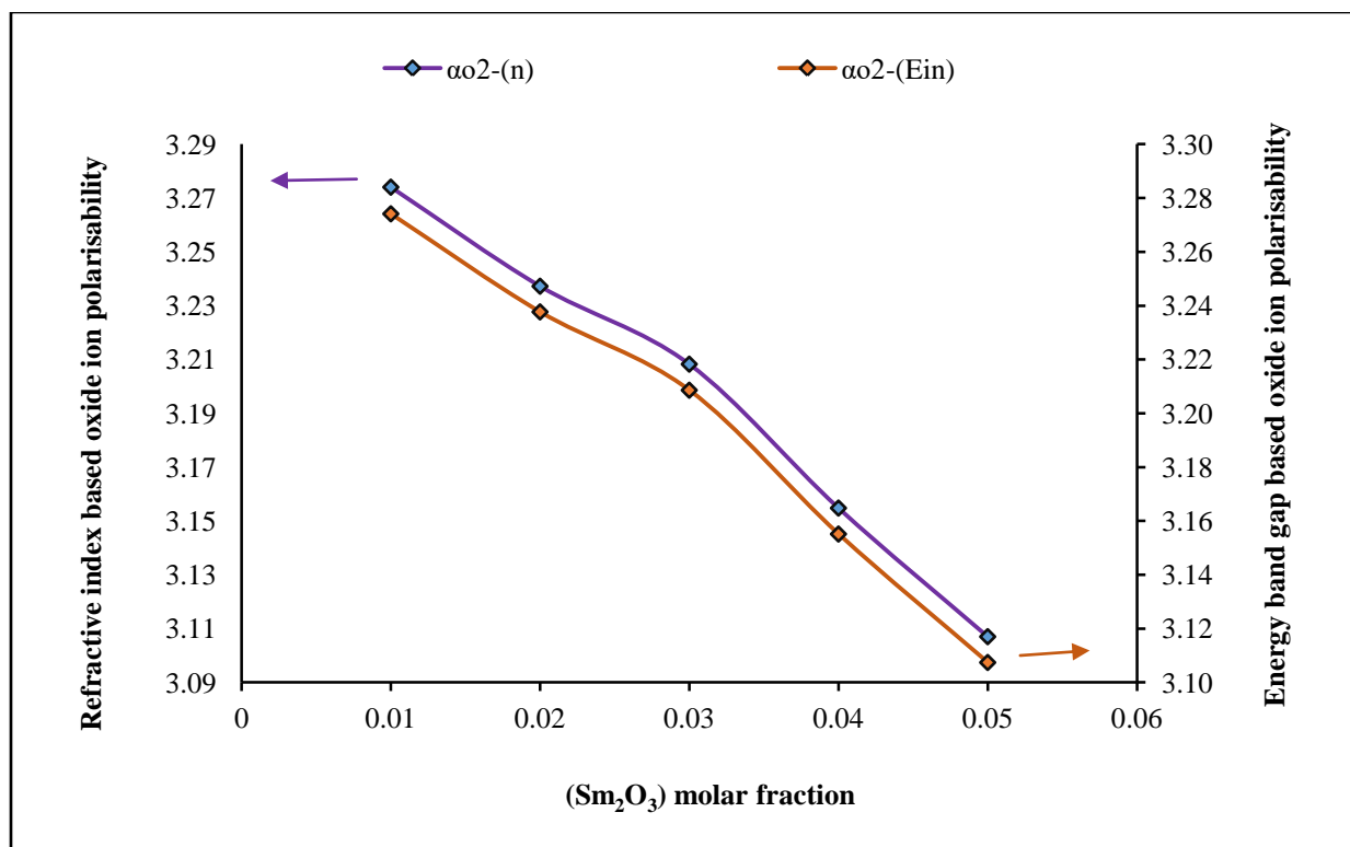
Figure 14: Oxide ion polarisability for [(TeO_2)_{0.7}(ZnO)_{0.3}]_{1-x}[Sm_2O_3]_x glasses.
