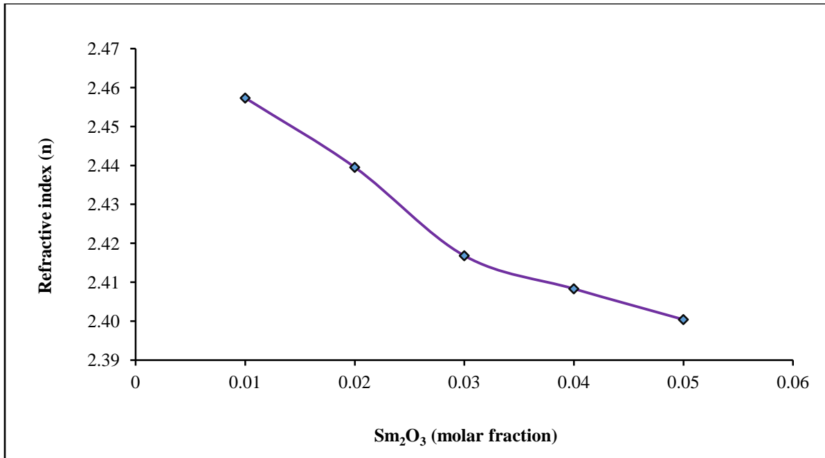
Figure 12: Plot of refractive index for [(TeO 2 ) 0.7 (ZnO) 0.3 ] 1-x [Sm 2 O 3 ] x glasses
